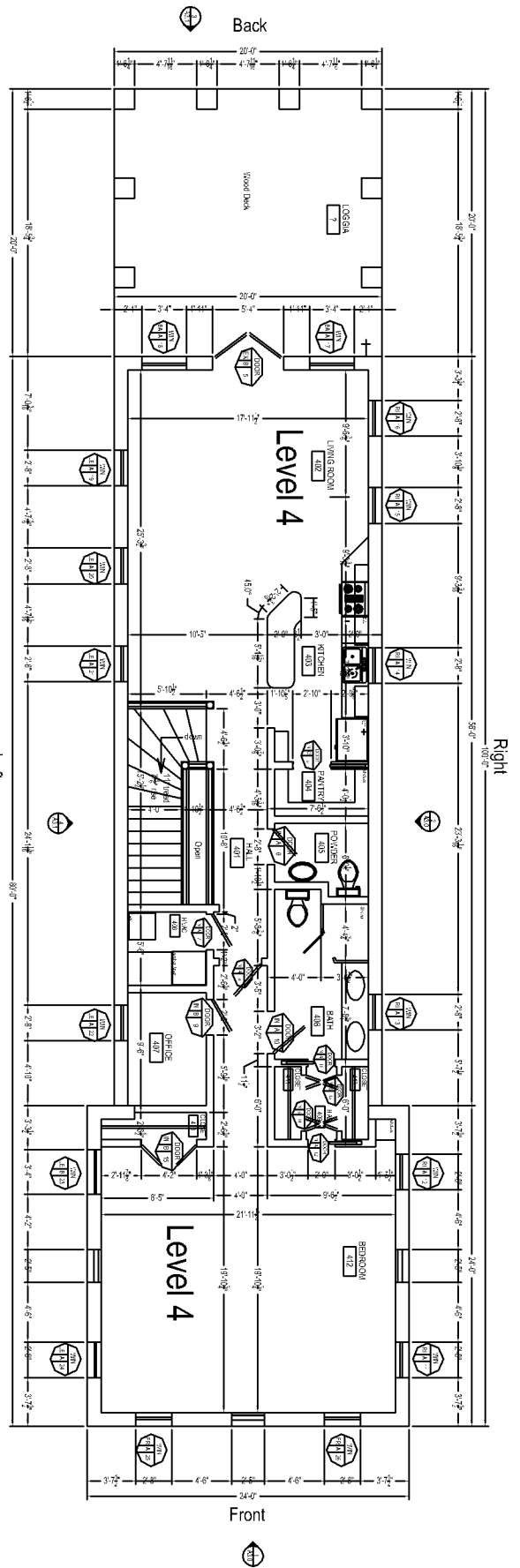
1 FLOOR PLAN - LEVEL 4 SCALE: 1/8" = 1'-0"
